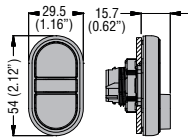
LPCB72... LPCBL72...
