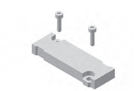
Blanking plate
