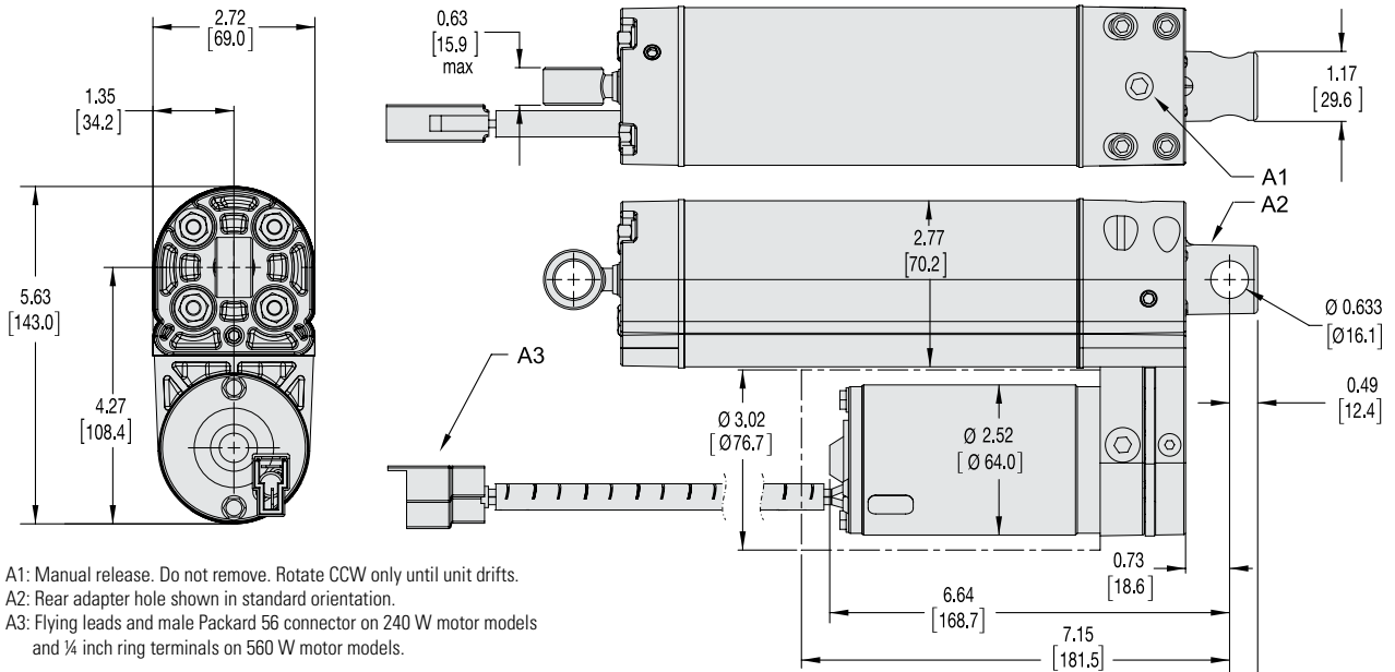
Type A front adapter
