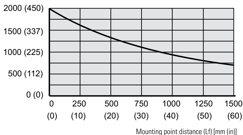
Maximum Permissible Deflection of Profile
