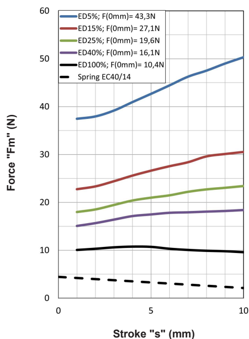
Force-stroke curve
