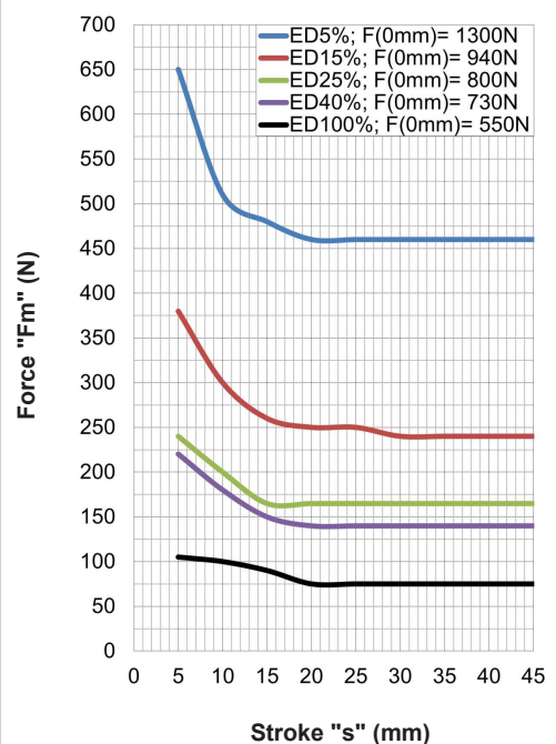
Force-stroke curve
