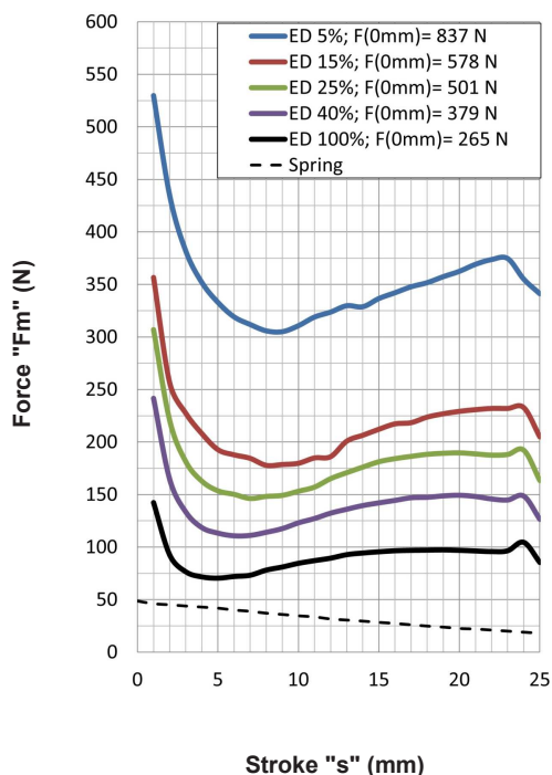
Force-stroke curve
