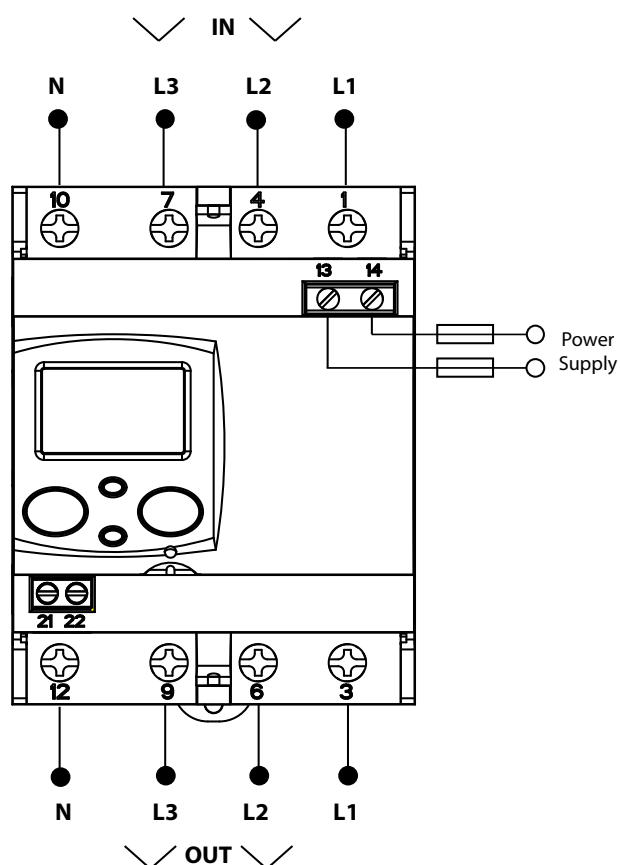
Figure 3: Connection diagram, CEM-C21.
