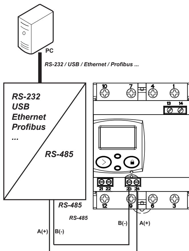
Figure 18: CEM-C21-485-T1 and CEM-C21-485-DS connection diagram.
