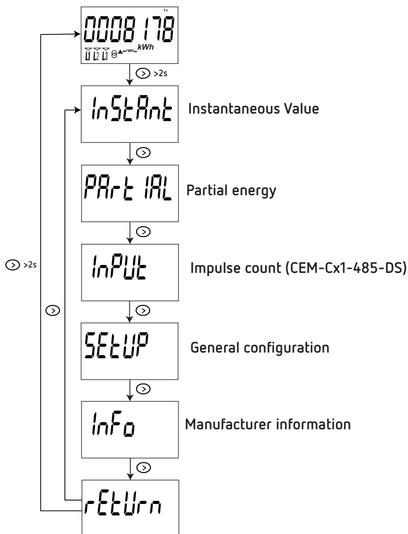
Figure 11: Navigation diagram in reading mode of the CEM-C21.
