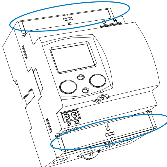
Figure 4: Terminal covers of the CEM-C21.
