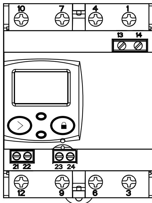
Figure 2:Terminals of the CEM-C21-485-T1 and CEM-C21-485-DS.
