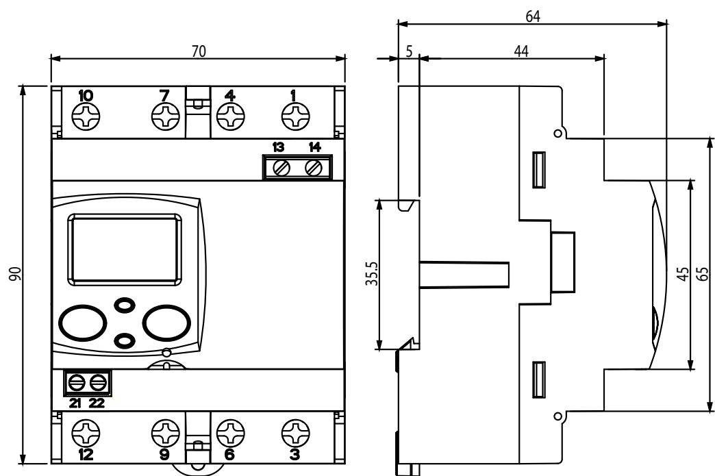
Figure 19: Dimensions of the CEM-C21.
