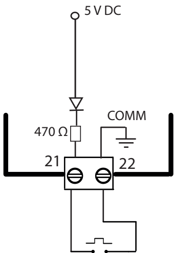
Figure 9: Digital input, CEM-C21-485-DS.
