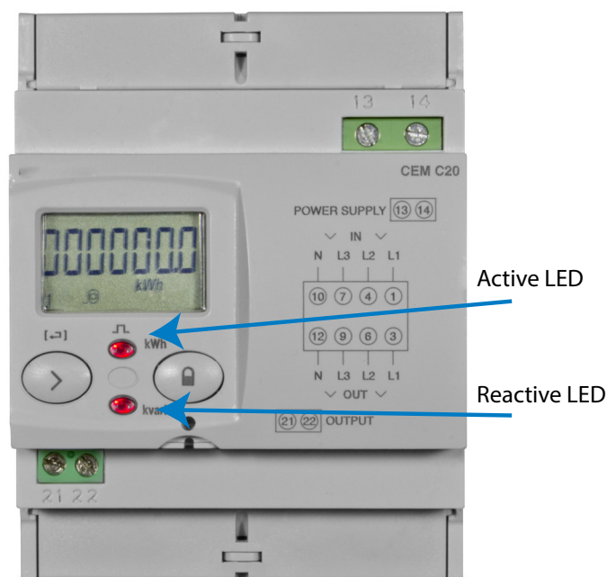
Figure 8: LED Indicators of the CEM-C21.
