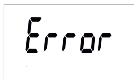
Figure 10: Error screen.
