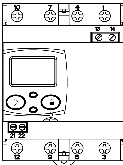
Figure 1: Terminals of the CEM-C21-T1.
