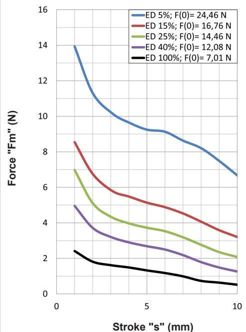
Force-stroke curve
