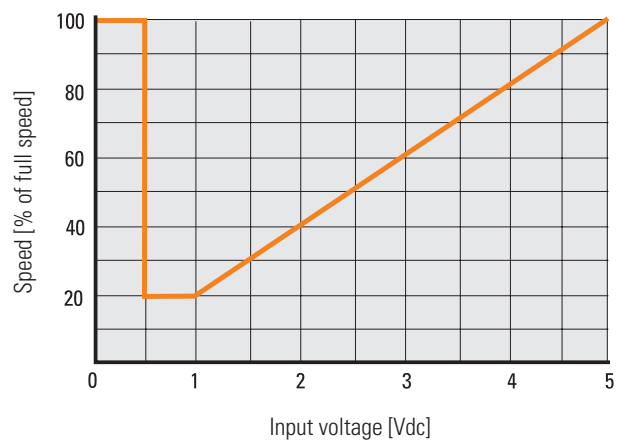
Speed vs. Speed Control Input Voltage
