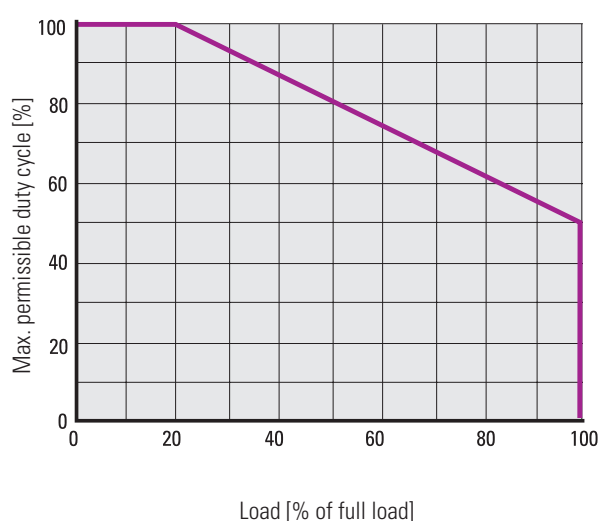
Duty Cycle
