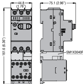
SM1P... with BG... mini-contactors and connection SM1X3040P
