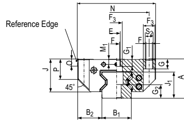
512 Style A
