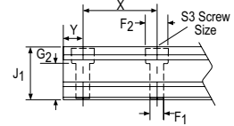
512 Style B
