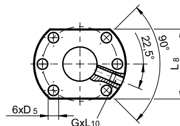
Hole pattern 1 according to DIN 69051
