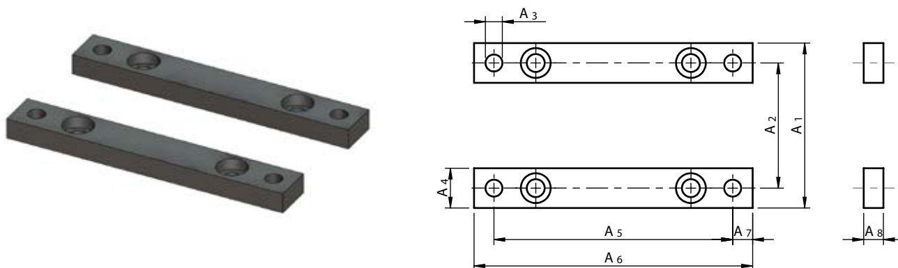
Dimensions [mm]
