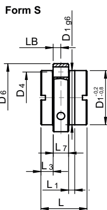
Hole pattern 1 according to DIN 69051
