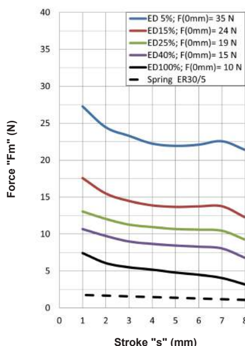
Force-stroke curve
