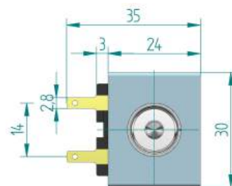
Solenoid under voltage (s=0mm position)
